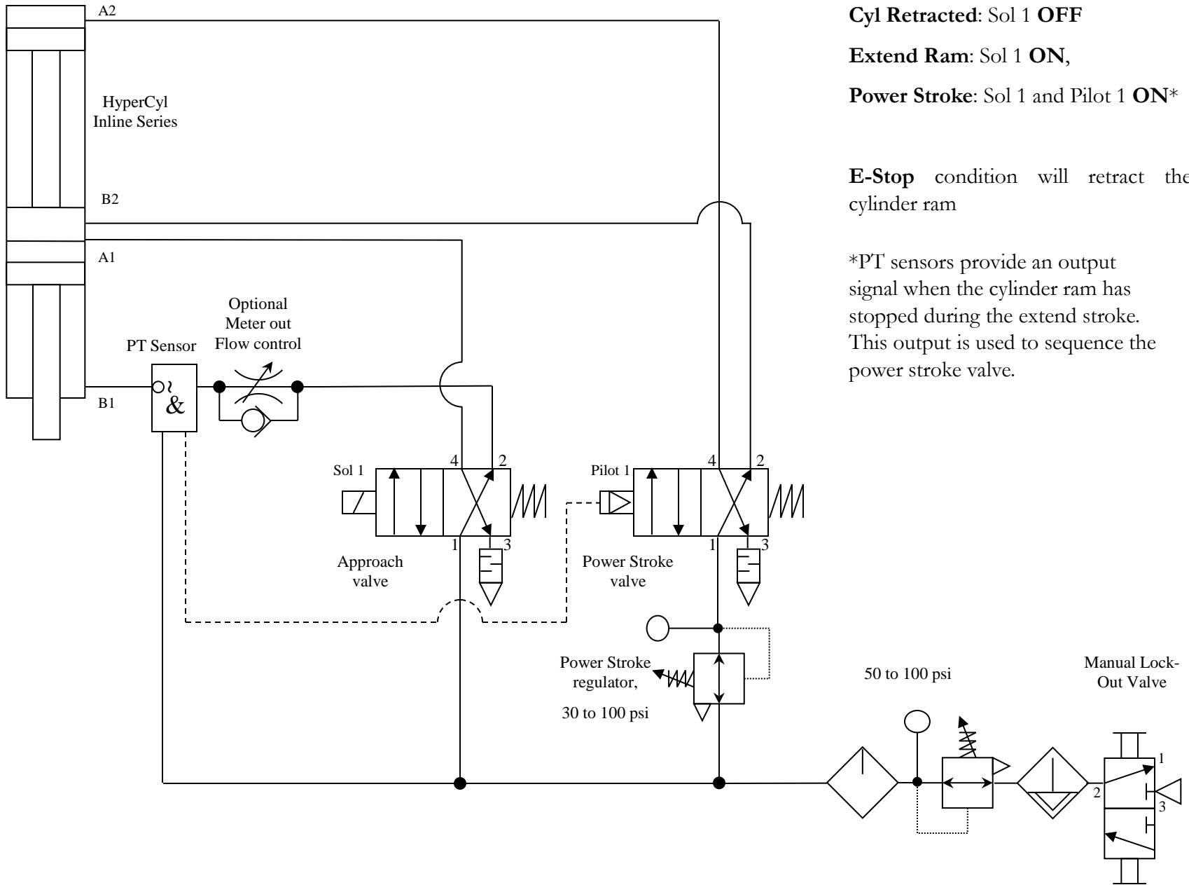
HPI 2-Position Spring Return PT Schematic
